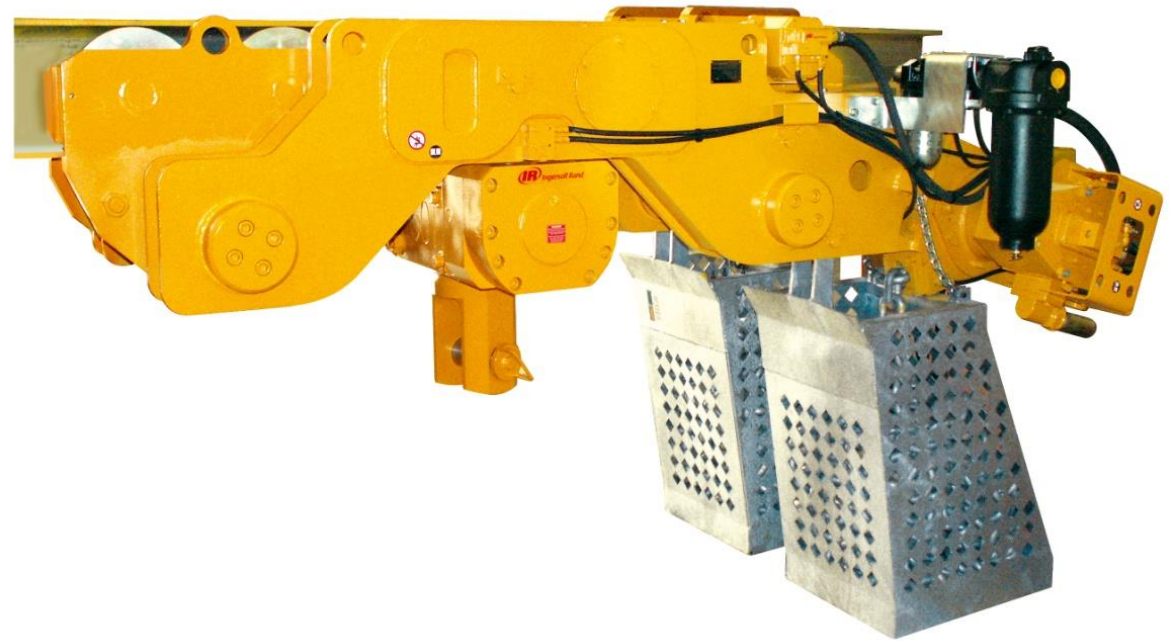
Ultra Low Headroom Trolley Hoist. SWL 50 ton
