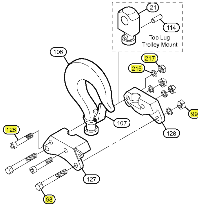
LC2A180T-LC2A250Q Top Hook and Trolley Mount Assembly Parts List
