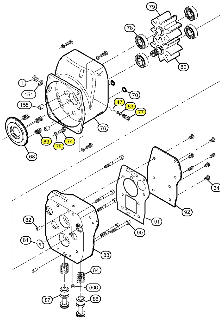
3.5HP Motor Assembly Without Emergency Stop Adapter Parts List
