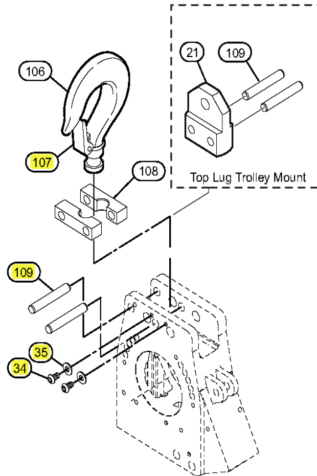
LC2A010S - 015S - 020D - 030D - 060Q Top Hook and Trolley Mount Assembly - Parts List (continued)
