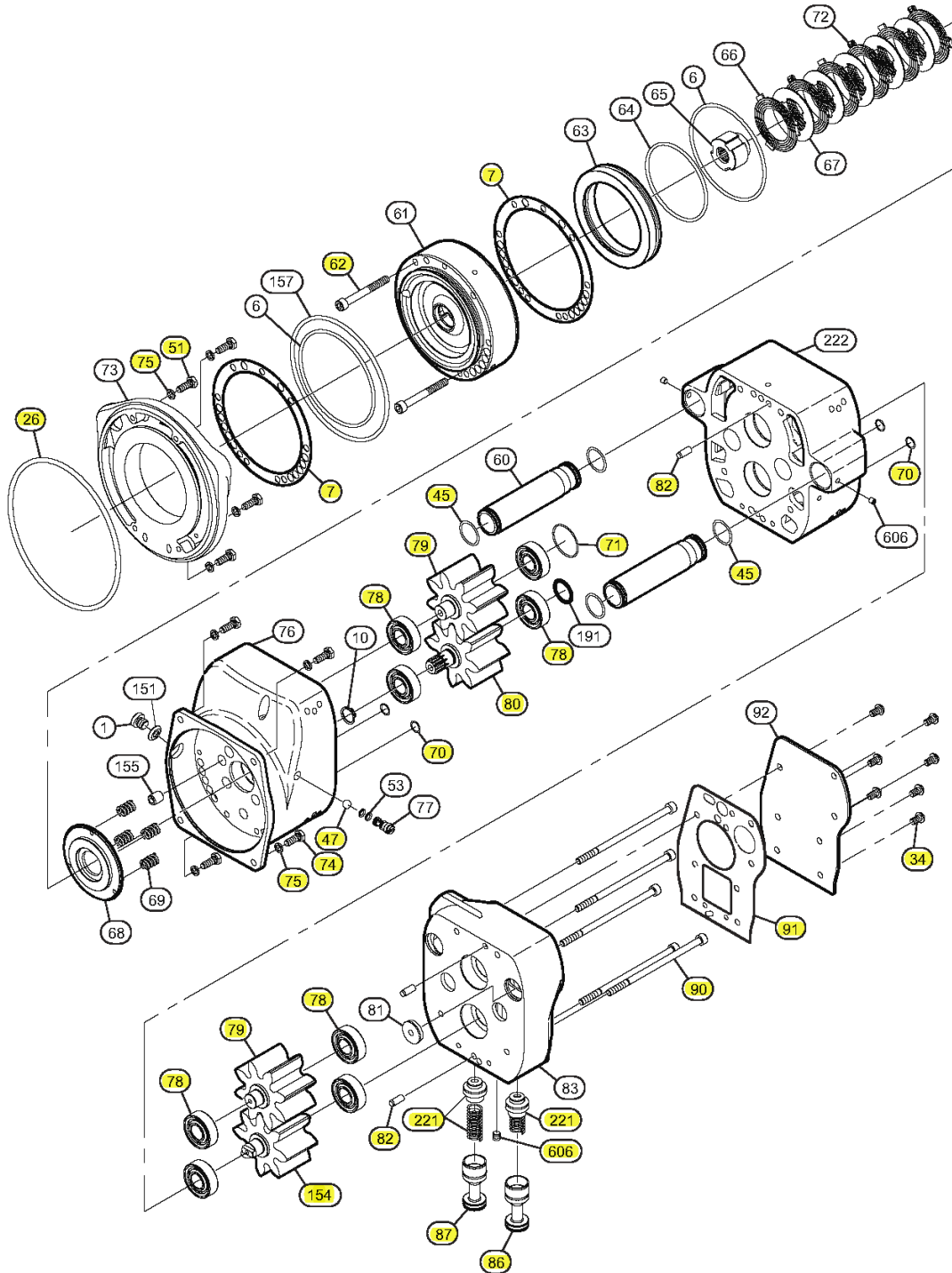
6HP Motor and Disc Brake Assembly Without Emergency Stop Adapter Parts List
