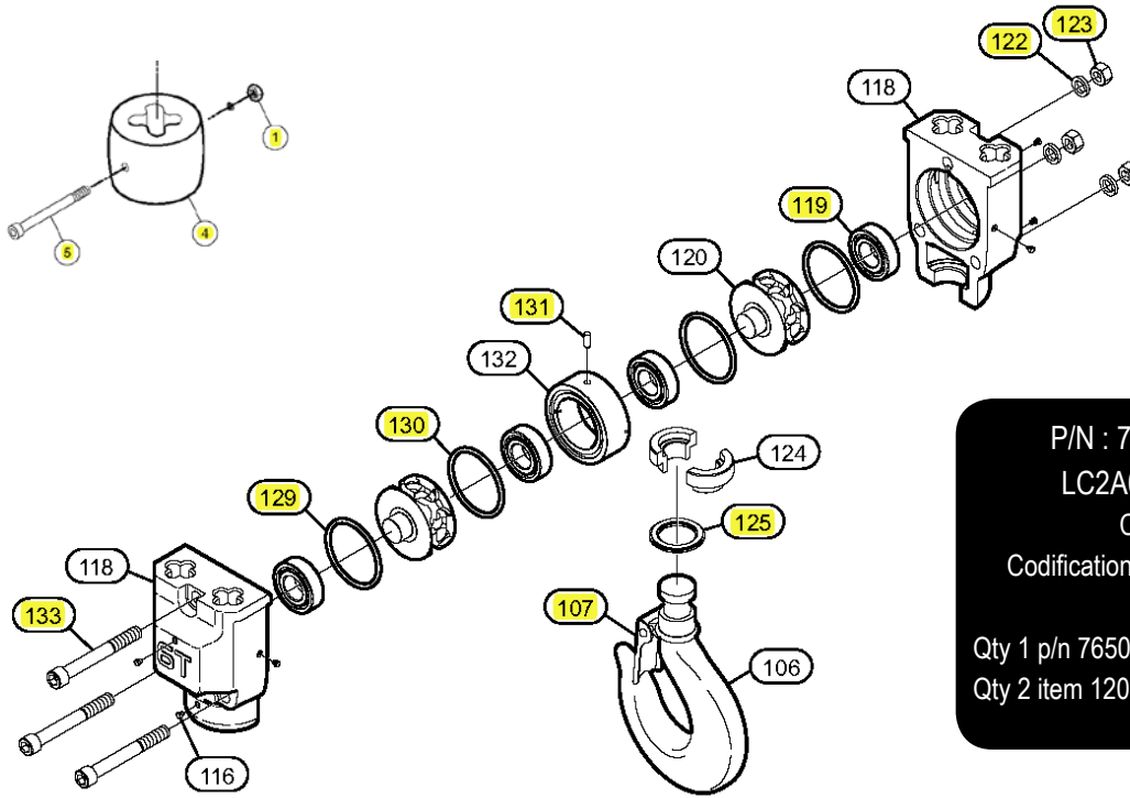
LC2A060Q Bottom Block Hook Assembly Parts List (continued)
