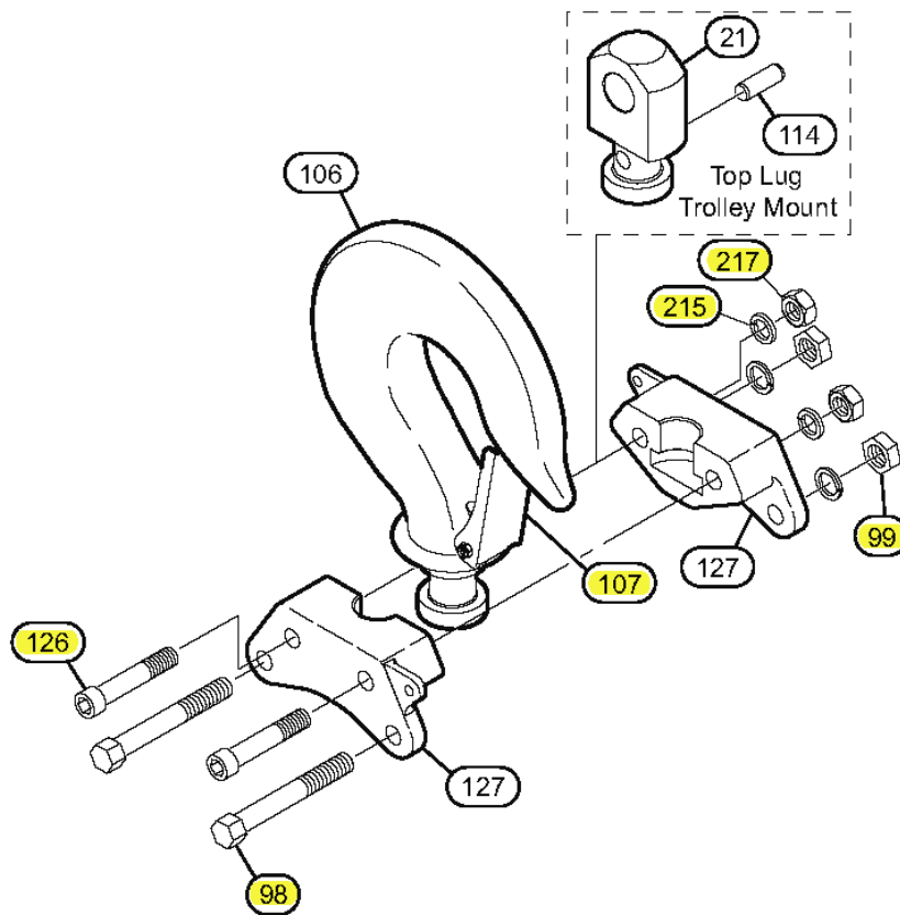
LC2A180T-LC2A250Q Top Hook and Trolley Mount Assembly Parts List
