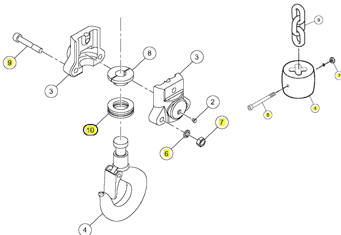
1T-1.5T Single Fall Capacity Bottom Block Assembly Parts List
