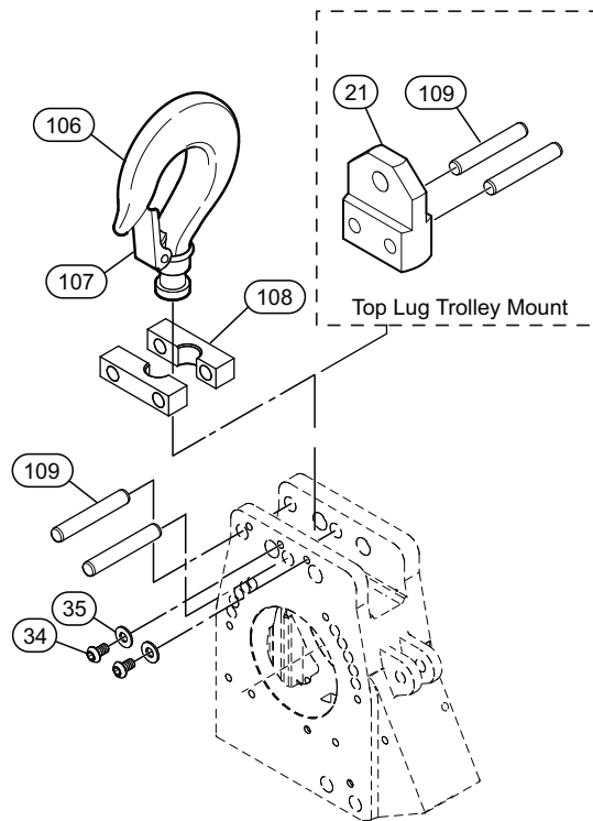
1.5 t single and 3 t Double Fall Capacity
